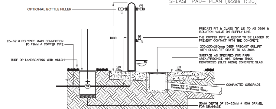
SPLASH PAD- PLAN (scale 1: 20)
